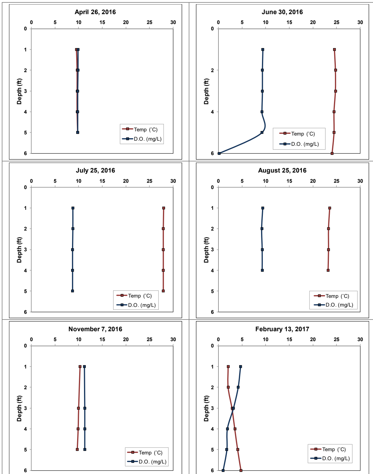
Figure 3.1-14. Gilkey Lake dissolved oxygen and temperature profiles.
