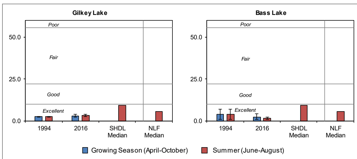
Figure 3.1-8. Gilkey and Bass Lakes, state-wide shallow headwater drainage lakes, and regional chlorophyll- a concentrations. Mean values calculated with summer month surface sample data. Water Quality Index values adapted from WDNR PUB WT-913.
