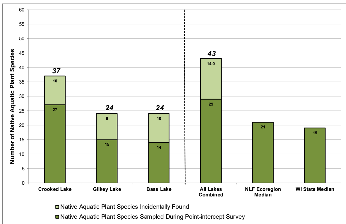
Figure 3.4-11. Crooked Lake Area Lakes species richness. Created using data from the August 2016 surveys. Analysis follows Nichols (1999).
