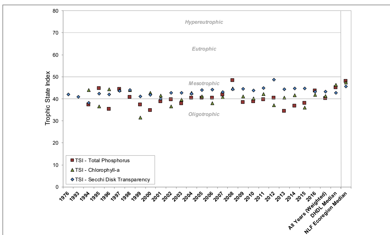
Figure 3.1-11. Crooked Lake, state-wide deep headwater drainage lakes, and regional Trophic State Index values. Values calculated with summer month surface sample data using WDNR PUB-WT-193.
