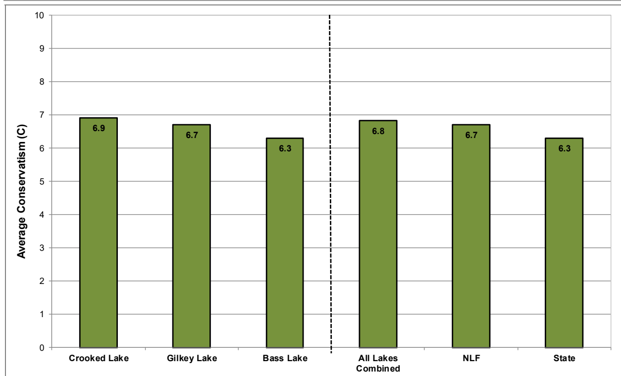
Figure 3.4-12. Crooked Lake Area Lakes average conservatism. Created using data from the August 2016 surveys. Analysis follows Nichols (1999).
