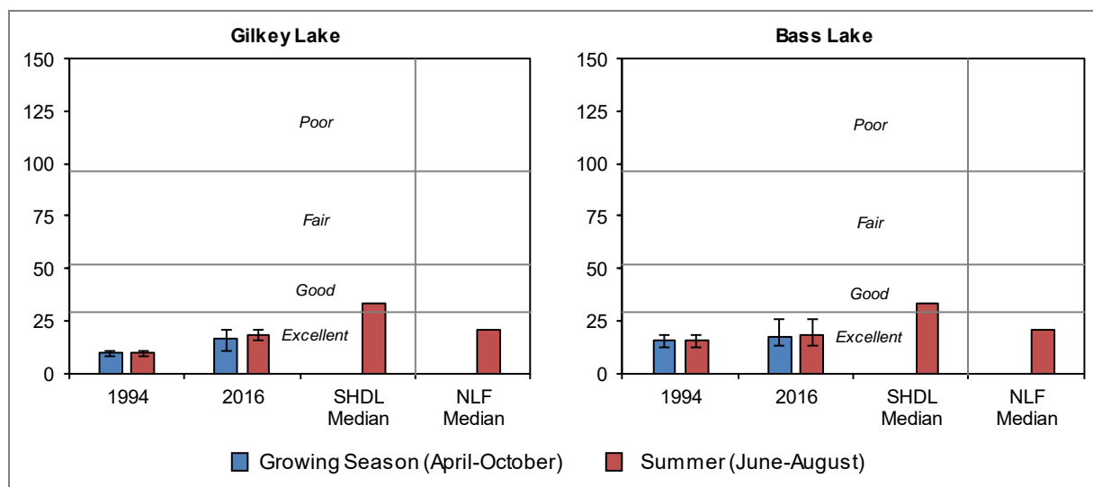
Figure 3.1-7. Gilkey and Bass Lakes, state-wide shallow headwater drainage lakes, and regional total phosphorus concentrations. Mean values calculated with summer month surface sample data. Water Quality Index values adapted from WDNR PUB WT-913.
