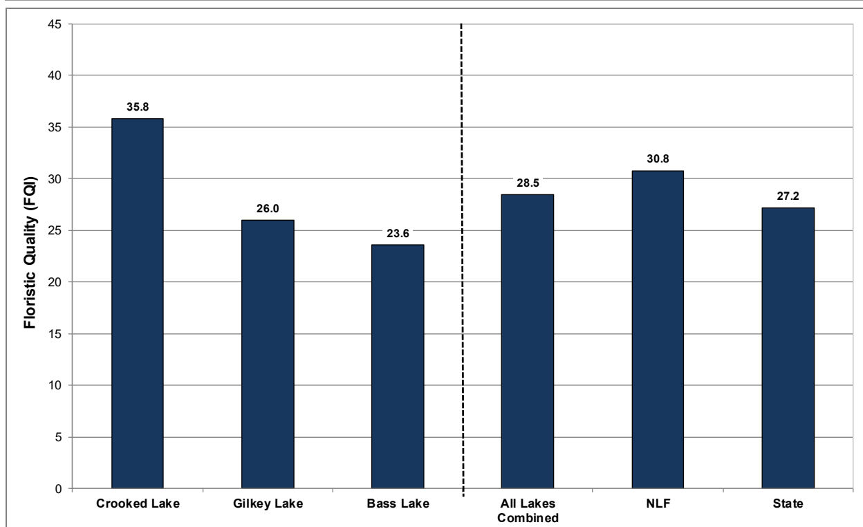
Figure 3.4-13. Crooked Lake Area Lakes Floristic Quality Index. Created using data from the August 2016 surveys. Analysis follows Nichols (1999).
