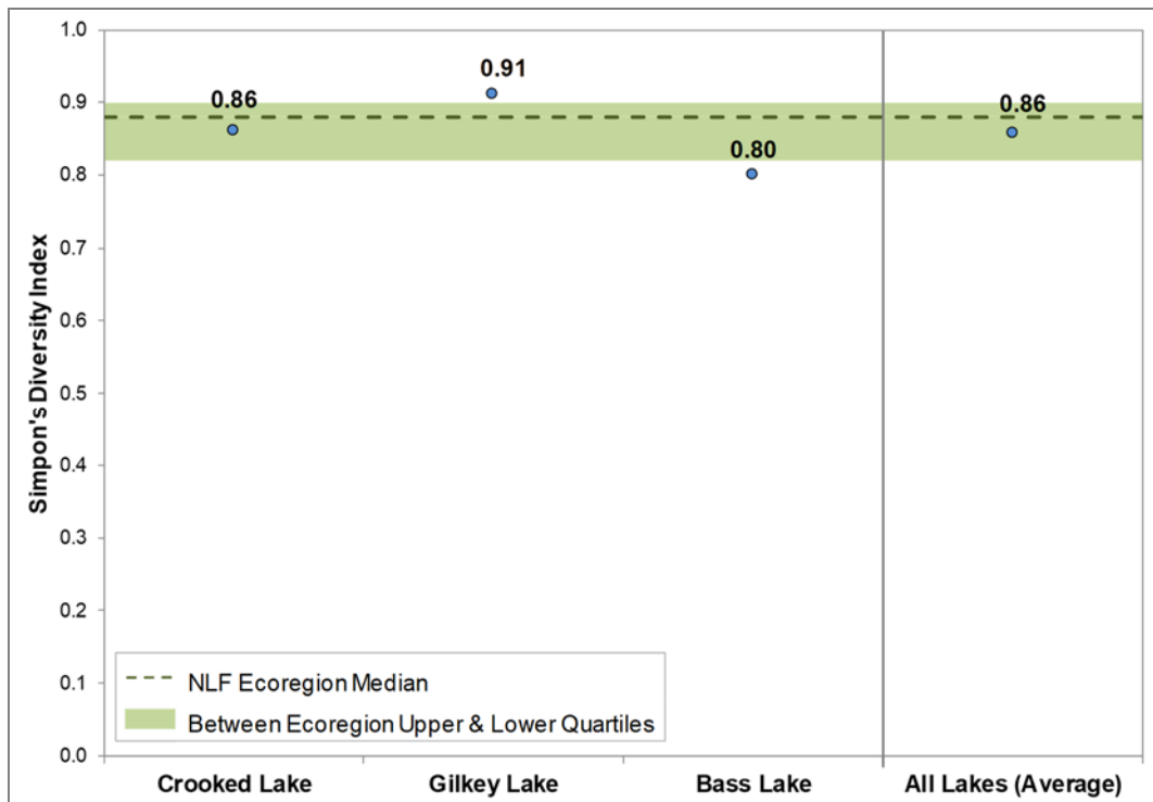
Figure 3.4-14. Crooked Lake Area Lakes species diversity index. Created using data from the 2016 aquatic plant surveys. Ecoregion data from 212 NLFL lakes collected by WDNR Science Services and Onterra.
